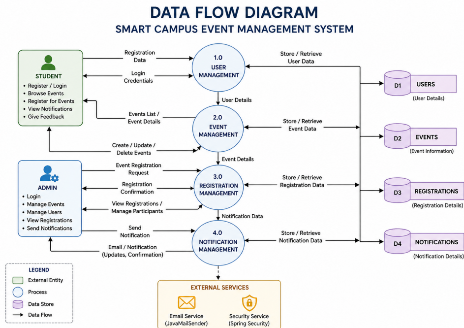
Figure 4.2: Data Flow Diagram
